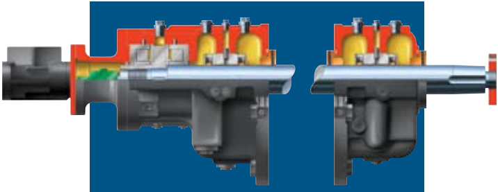
Split Sleeve Radial and Tilting Pad Thrust
