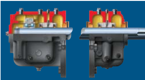
Split Sleeve Radial and Ball Thrust
